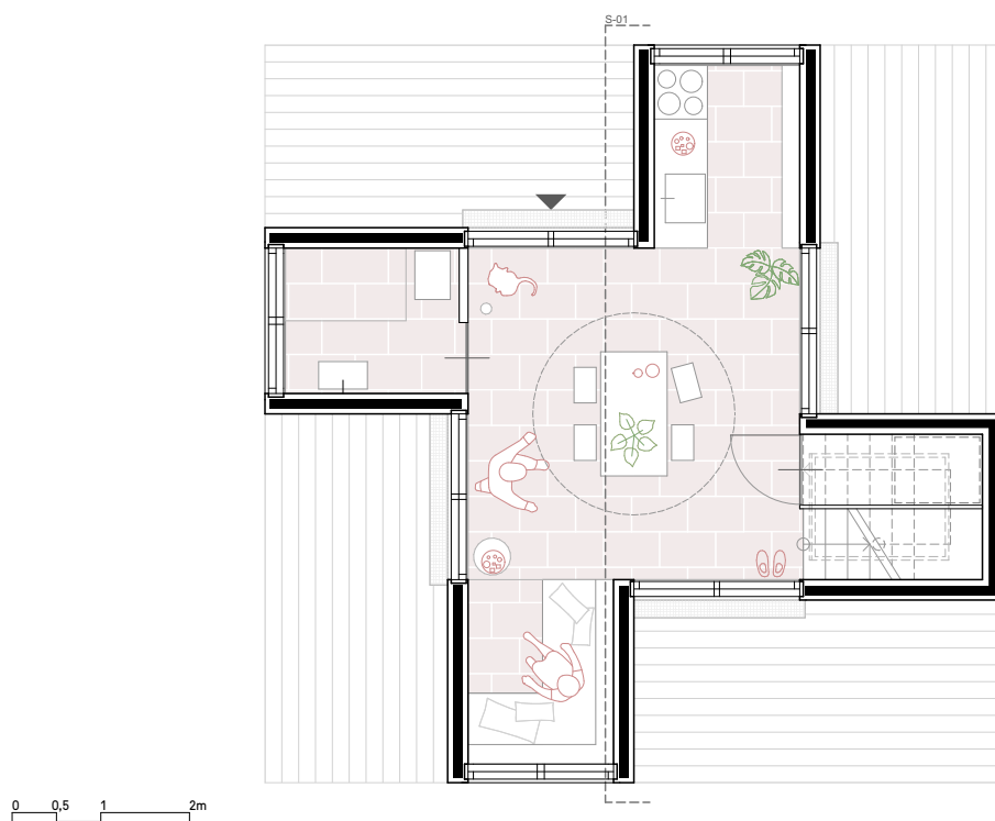
Grundriss Erdgeschoss Ground floor plan
