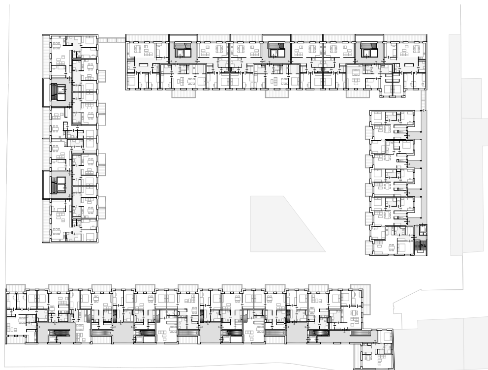
Grundriss 2.06 / Floor plan 2nd floor
