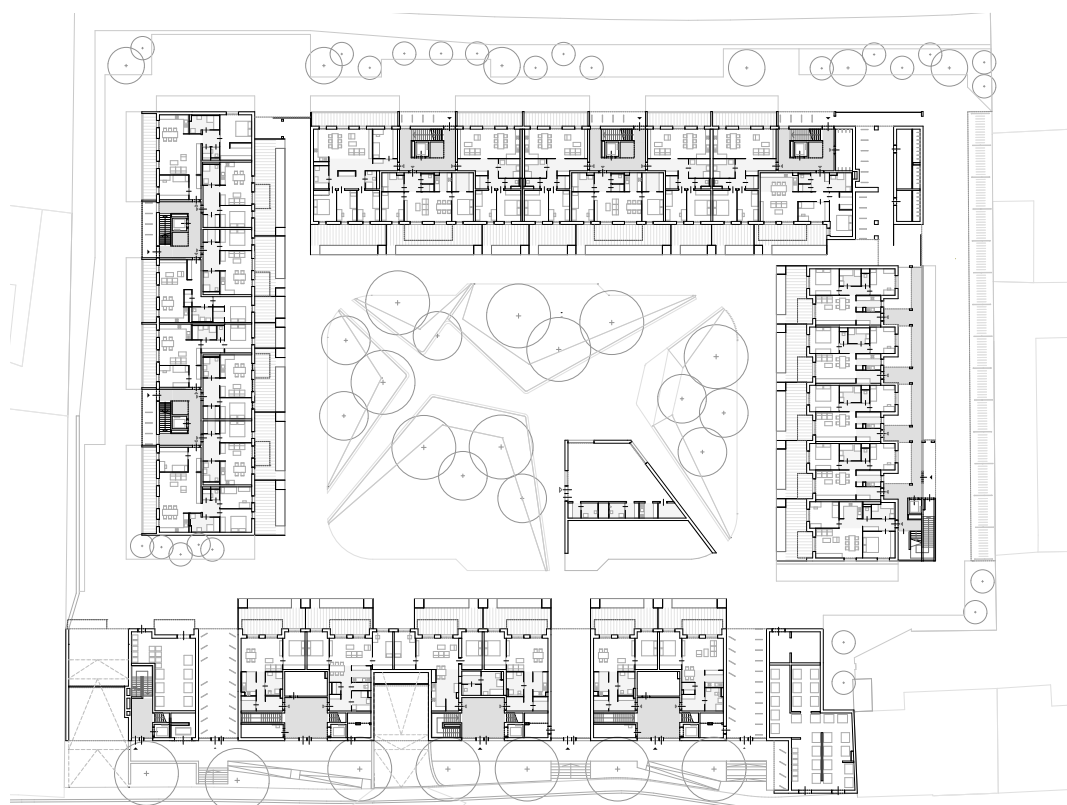
Grundriss EG / Ground floor plan
