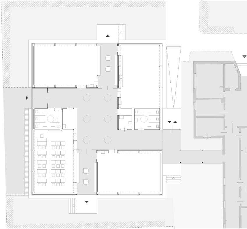
Grundriss Erdgeschoss Ground floor plan
